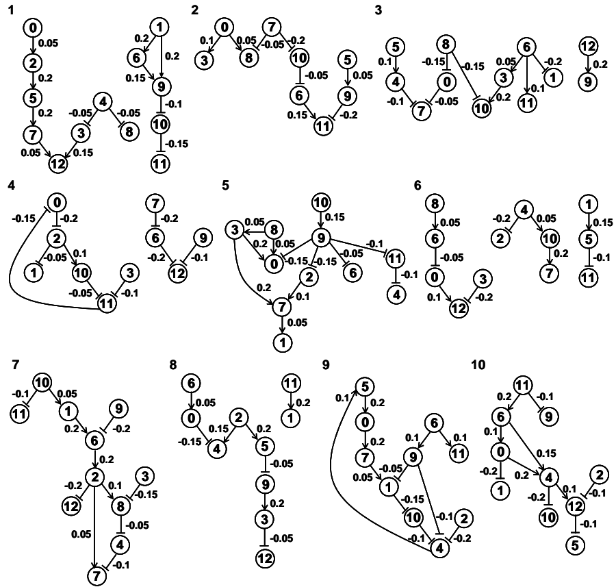
Supplemental Fig. 1. The 10 networks simulated by GeneSim to produce data sets. Numbers next to links specify regulation strengths. Arrows: activations; flat heads: repressions.
